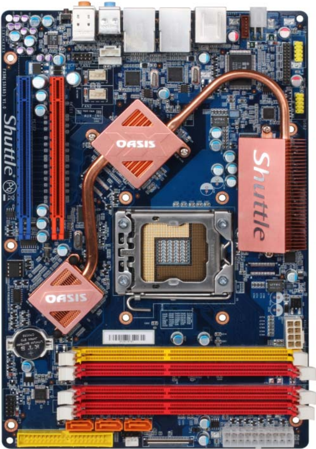
Mainboard of SX58J3:
